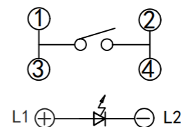
CIRCUIT
