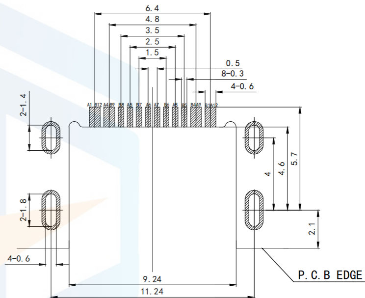
RECOMMENDED PCB LAYOUT (COMPONENT SIDE) TOLERANCE UNSPECIFIED ±0.05mm
